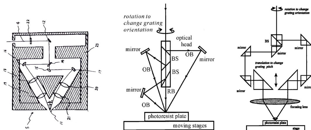
Left: Diagram of the dot-matrix system patented in 1984 by Iwata Fujiro of Toppan Printing Co. Ltd. which used two independently driven rotating mirrors to scan two beams through lenses, providing a variable spatial frequency only. Centre: Diagram of the optically complex Davis Light Machine, sold by Dimensional Arts Inc. from 1991. Right: Diagram of the even more optically complex C. K. Lee / Sparkle system, sold by Ahead Optoelectronics Inc. from 1998.
