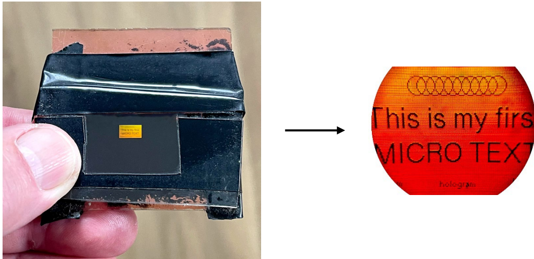
The second hologram test made in August 1996 – 1:1 scale. Thought to be the first dot-matrix hologram to contain microtext and micropatterns. The microtext recorded was just 80 \mu\text{m} (0.08 mm) high.
