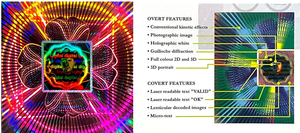
A sample multiple-resolution Lightgate dot-matrix security hologram, 2002, incorporating the features listed on the left. At its centre is a 3Digital holographic portrait of Rob Munday. This may have been the first digital holographic portrait created using a 3D digital scan of a person's head. The resulting 3D data was then used to construct the computer model from which the stereographic image sequence was rendered.
